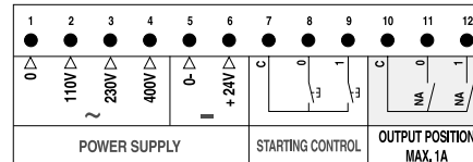
MO diagram
